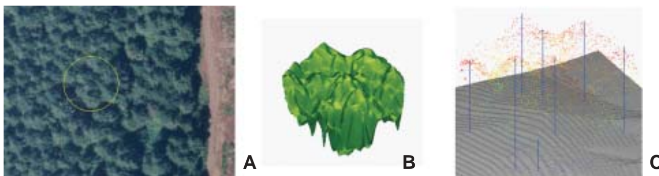
Figure 10-3—(a) Large-scale aerial photo showing growth plot, (b) detailed canopy surface model generated from LIDAR data, and (c) estimated individual tree stem locations and heights from LIDAR data.
