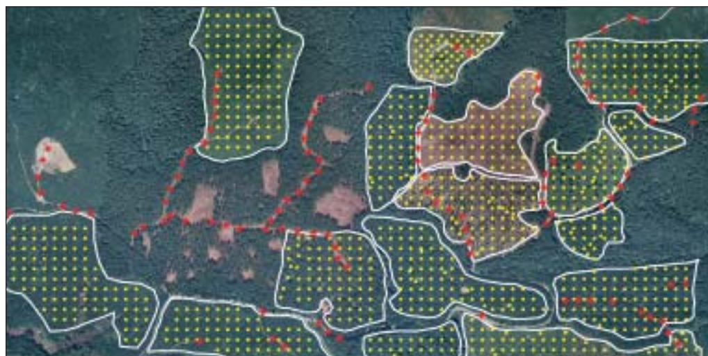
Figure 10-2—1999 orthophotograph showing location of 16 timber units in which photogrammetric spot heights were collected. Yellow dots represent spot heights in timber units. Red crosses represent spot heights on roads. (Washington State DNR, Resource Mapping Section.)
