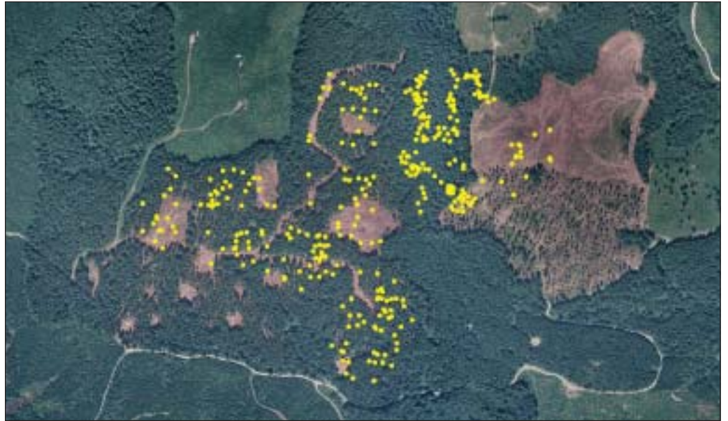
Figure 10-1—1999 orthophotograph of the LIDAR study area, after harvest. Yellow dots indicate the location of 350 ground survey checkpoints. (Washington State DNR, Resource Mapping Section.)
